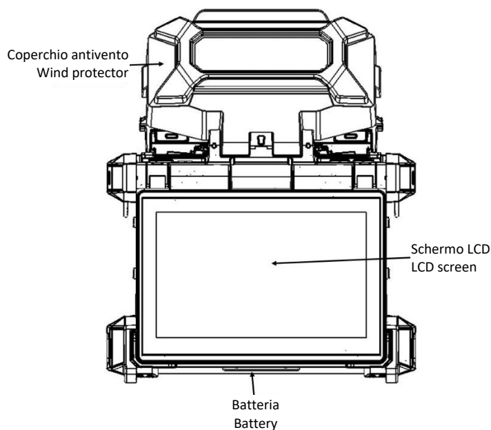
Vista frontale Frontal view
