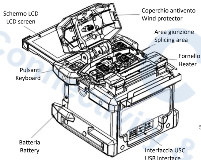
Vista isometrica Isometric view
